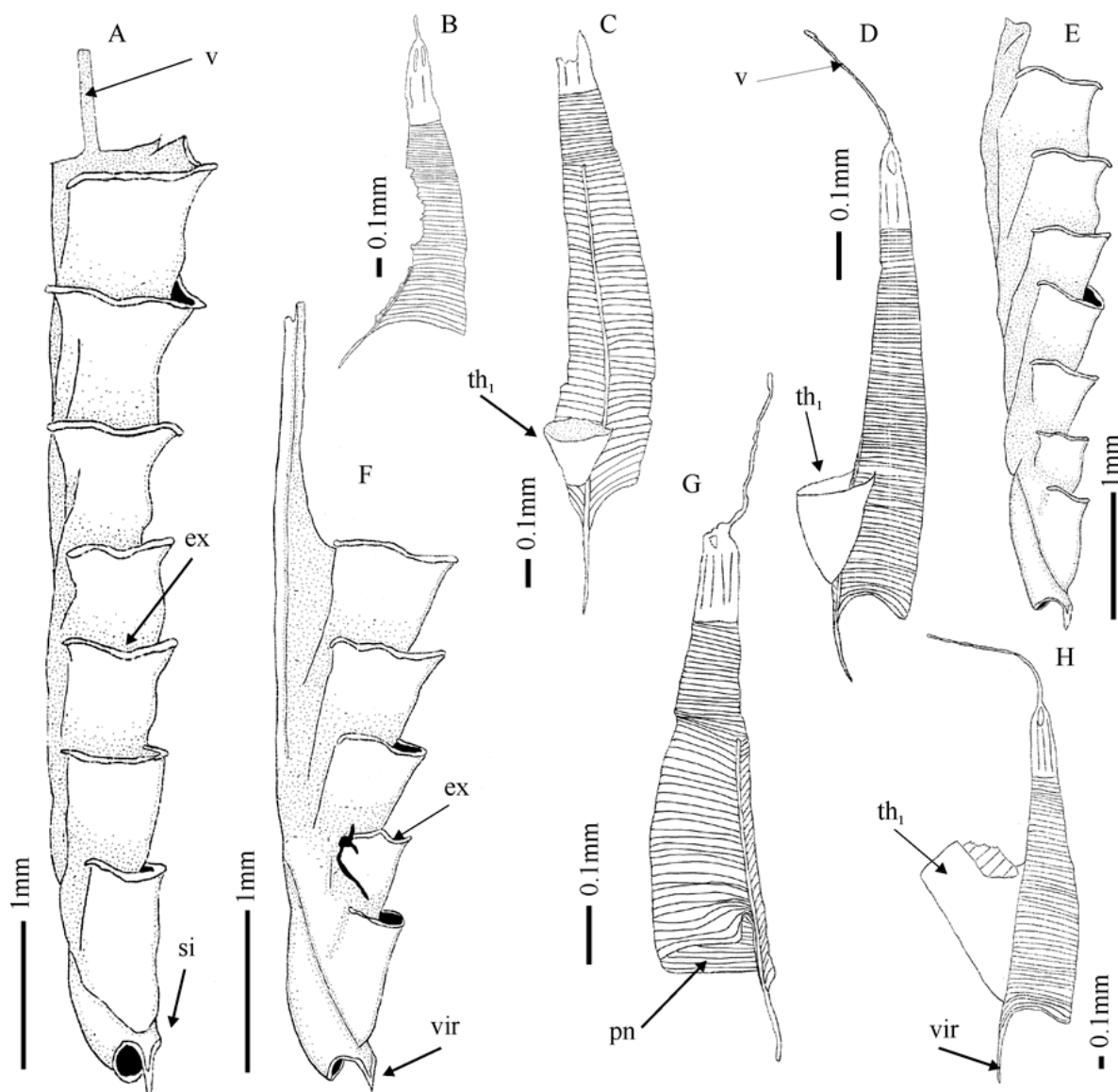
Figure 11: Pristiograptus lodenicensis PŘIBYL, all specimens from the Parovėja-9 borehole, A - P.P9-5, rhabdosome with virgula (v) and sícula (si); there is a small depression of the thecal apertural lip of th_3 (ex), depth 558.3m; B - P.P9-208a, sícula, depth 558.3m; C - P.P9-202a, sícula with beginning of th_1 ( th_1 ), depth 547.7m; D - P.P9-202b, sícula with incomplete th_1 ( th_1 ) and virgula (v), depth 547.7m; E - P.P9-6, proximal part of rhabdosome, depth 561.9m; F - P.P9-1, th_1 - th_5 , with a small depression on the apertural lip of th_2 (ex) and a virgella (vir), depth 561.9 m; G - P.P9-208b; sícula with open primary notch (pn), depth 558.3m; H - P.P9-208c sícula, virgella (vir) and th_1 ( th_1 ), depth 558.3m.
