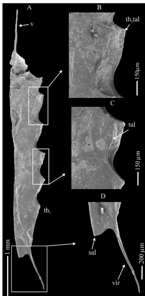
Figure 9: A-D Pristiograptus dubius var. "B", P.P222-216, Paežeriai-222 borehole, depth 734.5m. A - general view of proximal portion of a rhabdosome with virgella (v) and th_1 ( th_1 ); B - apertural lip of th_5 ( th_5tal ); C - end of the thecal apertural lip of th_2 (tal); D - sicula aperture with dorsal lip (sal) and long virgella (vir).
