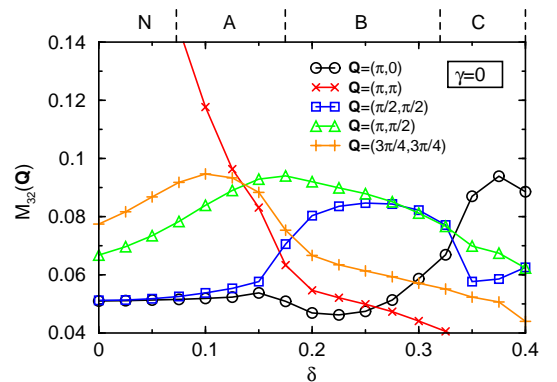
FIG. 10: (color online) Q dependent magnetic susceptibility obtained for the 32 sites cluster.
