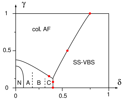
FIG. 3: (color online) Sketch of the phase diagram of the model (8). Phase transitions obtained by exact diagonalizations are indicated by full dots. The lines are guide to the eyes. The nature of the different phases is described in the following sections.
