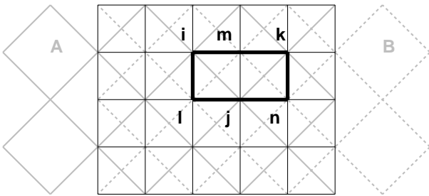
FIG. 1: Representation of a 3 by 2 horizontal rectangular plaquette. A vertical 2 by 3 plaquette can be obtained by a 90^\circ rotation of the plaquette. Gray plain and dashed lines represent the nearest-neighbor bonds of the A and B sub-lattices.
