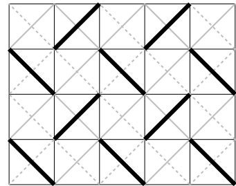
FIG. 2: Representation of one of the four ground states of model H_0 . Black lines indicate the pairs of spins that form singlet states. The three other ground states can be obtained by translation of the dimer pattern by lattice vectors.
