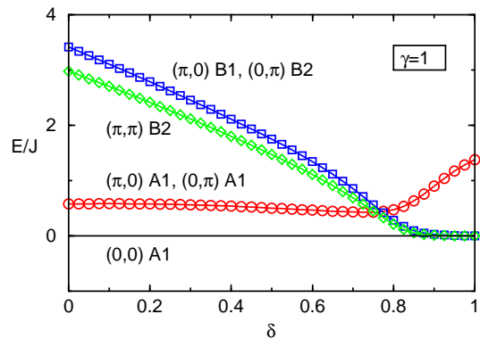
FIG. 5: (color online) Energy differences between the ground state and some of the lower states of the 32 site cluster. The symmetry of the different states is indicated on the figure. States with (\pi, 0) - A_1 and (0, \pi) - A_1 symmetry are triplet states, others are singlet states.
