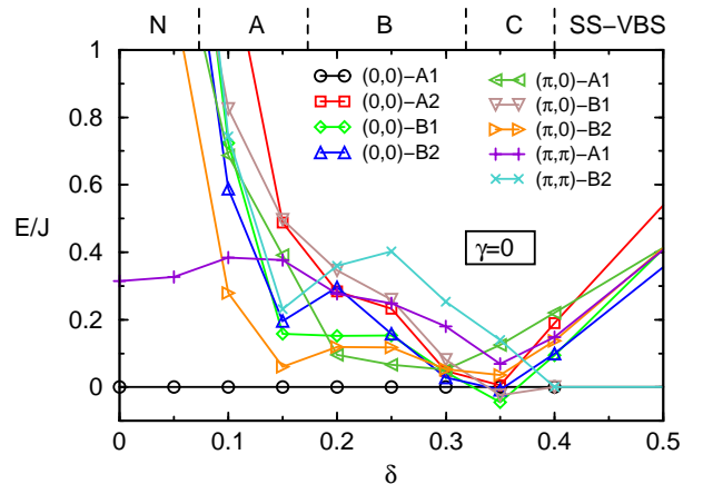
FIG. 8: (color online) Energy differences between the lower fully symmetric state with \vec{k} = (0, 0) momenta and some of the lowest states of the 32 site cluster. The symmetry of the different states is indicated on the figure.
