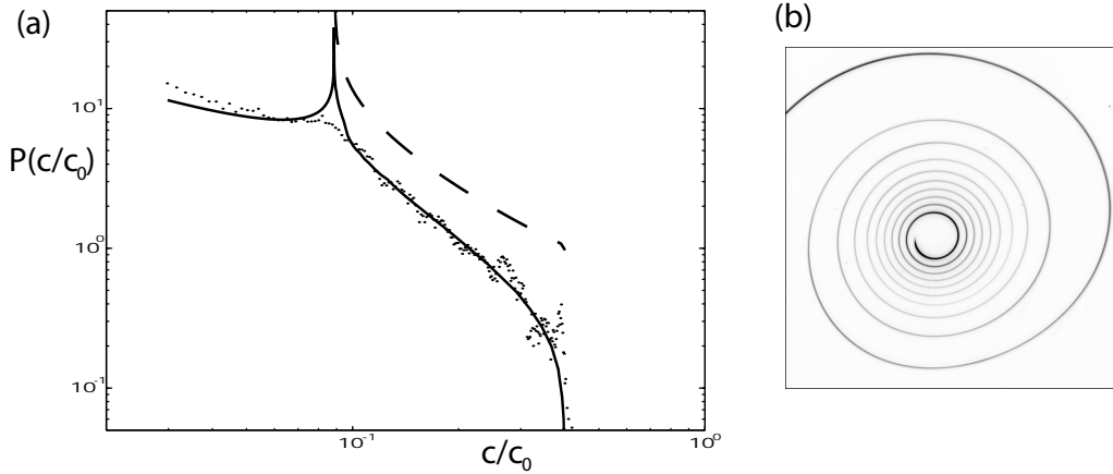
Fig. 2. (a) Probability density function of the concentration c and (b) concentration field at t = 60 s. . The solid line corresponds to the full model (4) and the dashed line to the approximation (6) using the maximal concentration.
