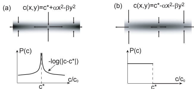
Fig. 3. Schematic of the singularities occurring in the scalar PDF of a 2D flow. (top) Pseudo-color plot of the scalar distribution c(x, y) . (bottom) The PDF is computed using P(c) = 4 \int_0^{R/\sqrt{\alpha}} |\partial c / \partial y|_{y_0(x)}^{-1} dx , with y_0(x) = \sqrt{c^* - c + \alpha x^2} / \sqrt{\beta} for (a) and y_0(x) = \sqrt{c^* - c - \alpha x^2} / \sqrt{\beta} for (b).
