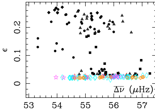
Fig. 11. Seismic quantity \epsilon characterizing the model evolutionary stage versus the mean large frequency spacing \Delta\nu . Grey open symbols indicate MS models, dark filled symbols PoMS models. Diamond 1.36 M_{\odot} , circle 1.38 M_{\odot} , triangle 1.42 M_{\odot} , stars 1.44 M_{\odot} , square 1.45 M_{\odot} , diamond 1.46 M_{\odot} , cross 1.48 M_{\odot} .
