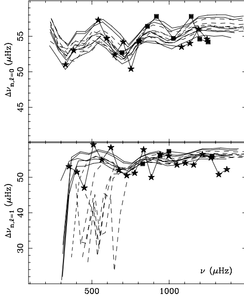
Fig. 10. Large frequency spacings for \ell = 0 (up) and \ell = 1 (down) for MS/PoMS models (full/dashed line) compared to Martić (stars) and Eggenberger (square) observations.
