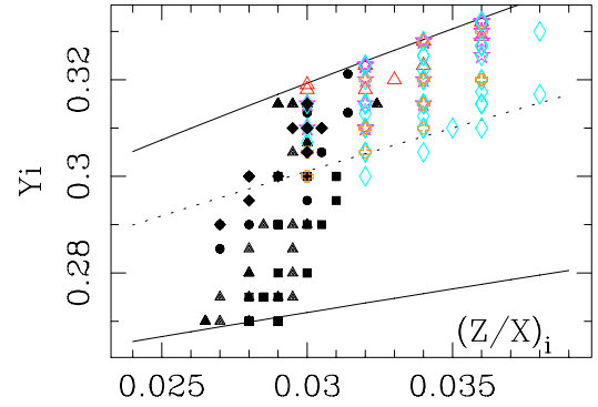
Fig. 4. Initial chemical composition of our models for Procyon A satisfying the constraints of Table 1. Grey open symbols indicate MS models, dark filled symbols PoMS models. Diamond 1.36 M_\odot , circle 1.38 M_\odot , triangle 1.42 M_\odot , stars 1.44 M_\odot , square 1.45 M_\odot , diamond 1.46 M_\odot , cross 1.48 M_\odot . The two full lines indicate the minimum and maximum values of Y_i resulting from the constraint of the galaxy chemical evolution given in Table 1. The dotted line corresponds to a stronger constraint \Delta Y / \Delta Z \leq 3 .
