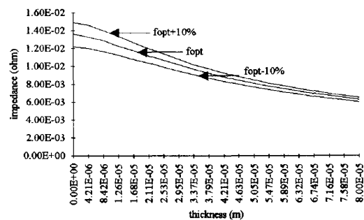
Fig.3. frequency influence
