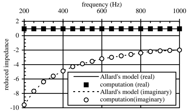
Fig. 4. Normal surface impedance of a porous material.
