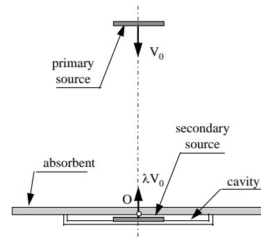
Fig. 5. Experimental set-up for the minimization of the acoustic pressure behind a porous material.
