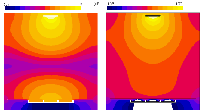
Fig. 8. Acoustic pressure in presence of a porous material at 200 Hz. Left: without control, right: with local impedance active control
