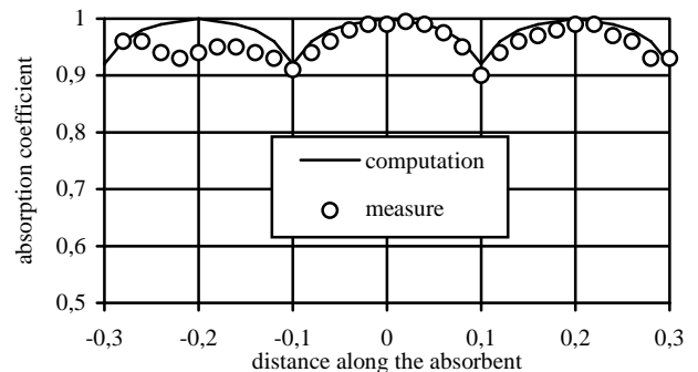
Fig. 9. Absorption coefficients along the absorbent - f = 200 Hz.
