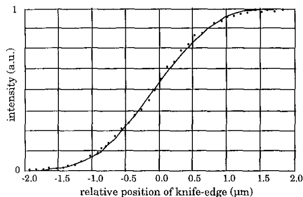
Figure 2. Determination of the beam profile by scanning a knife edge through the beam. Intensity is scaled to 1 for the knife edge out of the beam. The full line corresponds to a theoretical fit. After P. Engström (reported by Riekel et al. in Ref. [8]).
