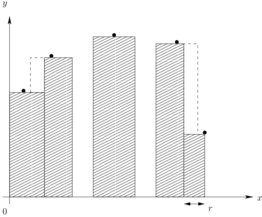
Figure 1: Hachured domain of “potential erasers” of \{(\widehat{x}_i, y_i), 1 \leq i \leq 5\} (black points)
