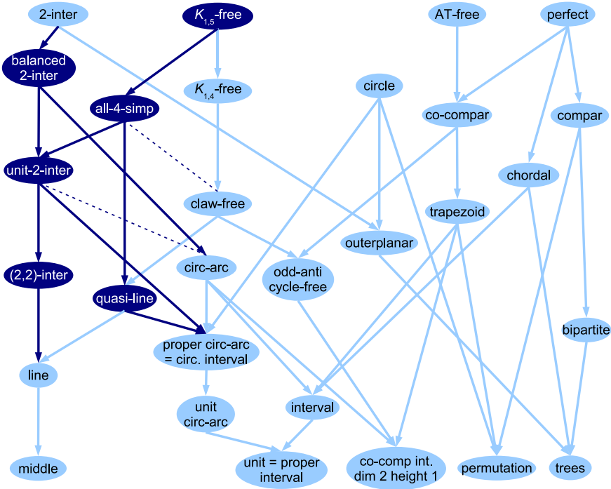
Figure 2: Graph classes related to 2-interval graphs and its restrictions. A class pointing towards another strictly contains it, and the dashed lines mean that there is no inclusion relationship between the two. Dark classes correspond to classes not yet present in the ISGCI Database [BLS + ].
