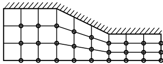
Figure 4: Coarse nodes for the die problem with n = 27 subdomains
