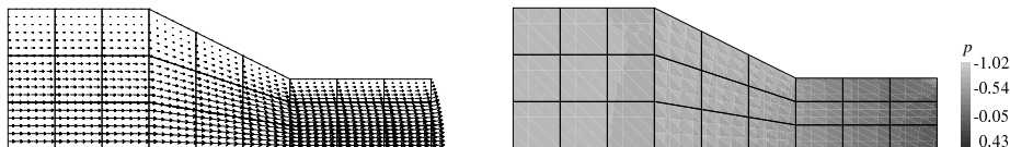
Figure 3: Solution to the die problem with n = 27 subdomains and h/H = 1/6 ; left: displacement field, right: field of variable p
