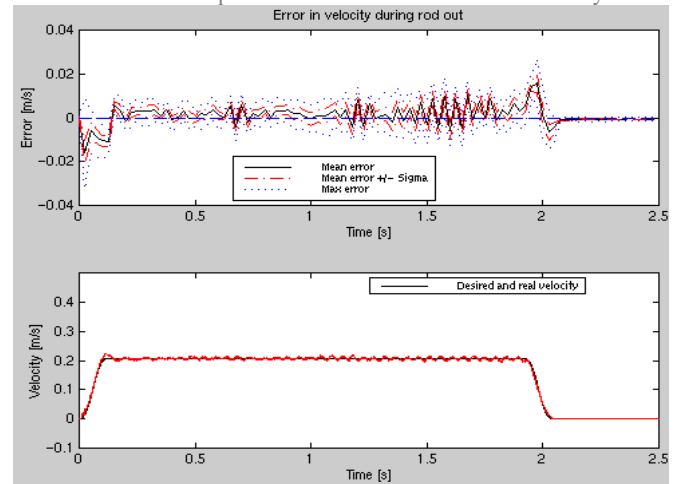
b Nonlinear control results Fig.21 Error in velocity.
