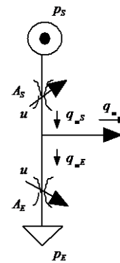
Fig. 2 Wheatstone half bridge representation.
