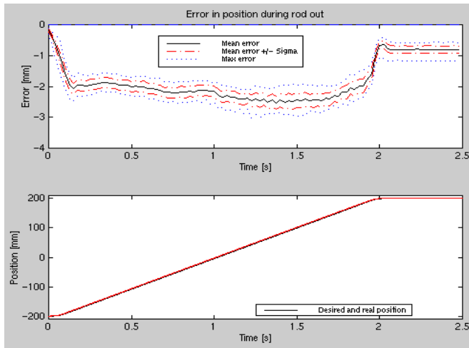
b Nonlinear control results Fig.20 Error in position.
