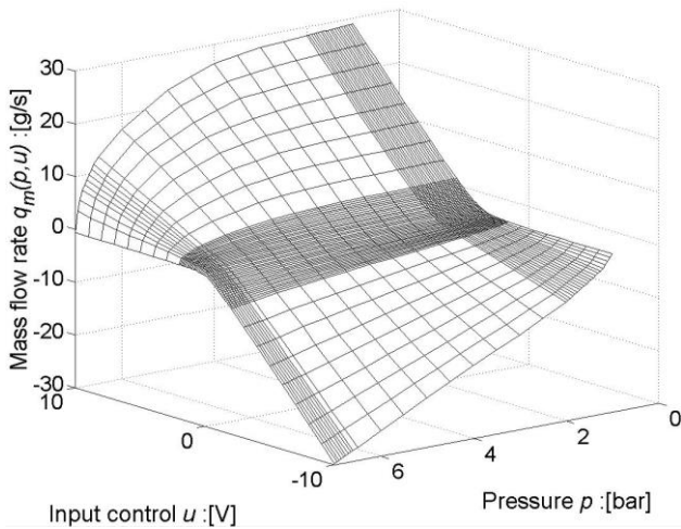
Fig. 3 Servo-distributor static characteristics.
