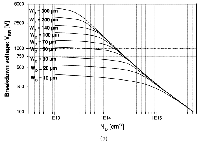
Fig. 8. (a) Simulation circuit for breakdown voltage estimation. (b) Estimated breakdown voltage using the 1-D model in Fig. 1.
