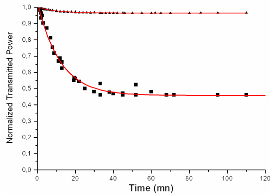
Fig. 3. Transmission of 633 nm and 1064 nm signals as a function of exposure time to pump light, the solid lines represents an exponential fit to the data.
