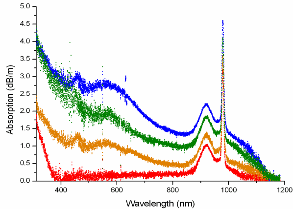
Fig. 1. Absorption spectra of a new Yb-doped LMA fiber (lower curve, red) and of the same fiber at different states of photodarkening at 7 min, 15 min and 100 min (upper curves, orange, green and blue) of pumping the fiber by light of 45 W at 976 nm.
