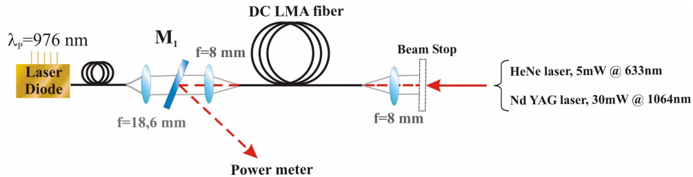
Fig. 2. Experimental setup for the transmission signal pump-probe experiment: M_1 is a dichroic mirror ( T_{\max} @ \lambda=980 nm and R_{\max} @ \lambda=1.06 \mu\text{m} ).
