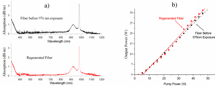
Fig. 6. (a). Absorption spectrum of a new (black line, upper graph) and a photobleached (red line, lower graph) fiber and (b). output characteristics of the cw LMA fiber laser oscillator using the same fiber, new (black circles) and photobleached (red squares).
