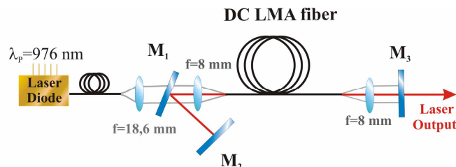
Fig. 4. Experimental setup of the LMA fiber laser. M_1 is a dichroic mirror ( T_{\text{max}} @ \lambda=980 \text{ nm} and R_{\text{max}} @ \lambda=1.06 \mu\text{m} for i=22.5^\circ ), M_2 is a high reflecting mirror at \lambda=1.06 \mu\text{m} , and M_3 is a dichroic mirror ( T_{\text{max}} @ \lambda=1.06 \mu\text{m} and R_{\text{max}} @ \lambda=980 \text{ nm} ) that served to eliminate the residual pump light.
