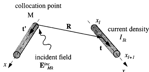
Fig. 1. Contribution of a straight segment at the collocation point M .
