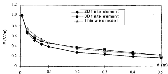
Fig. 5. Comparison of the scattered field between 2D FEM, 3D FEM and our model along a line perpendicular to the wire (Fig. 4).
