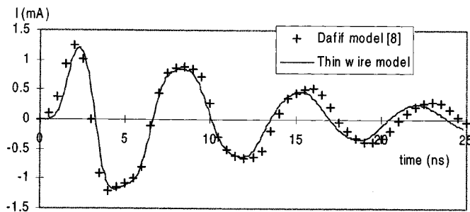
Fig. 6. Current induced in a thin wire antenna ( L = 1 m, a = 6.7 mm) E^{inc} = \exp[-a_0^2(t - t_{max})^2] , with a_0^2 = 24.95c^2 and t_{max} = 0.52/c .
