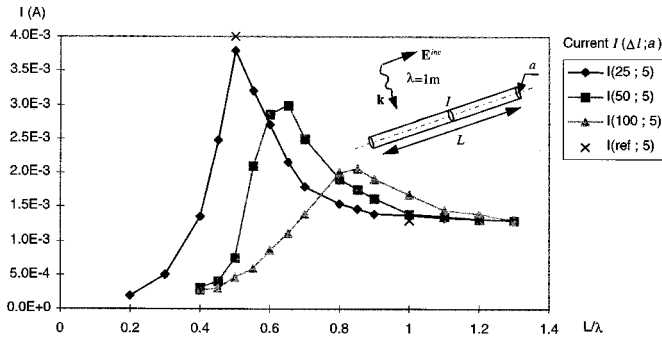
Fig. 2. Current induced by a 1 V/m-300 MHz incident electric field at the middle of a wire antenna for a radius a = 5 mm for several values of L and \Delta l . Reference values (denoted ref) are presented in [6].
