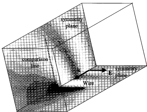
Fig. 4. Scattering by a thin wire antenna ( L = 1 m, a = 5 mm) for a 1V/m-300 MHz incident plane wave. Computation by 3D finite element method [7]. Visualization of the total field in the symmetry planes.
