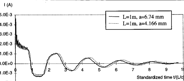
Fig. 7. Current at the center of a 1 m wire antenna for two different radii. The antenna is fed by a 1 V voltage step.
