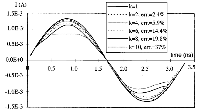
Fig. 3. Current induced at the middle of a straight antenna ( L = 1 m, a = 5 mm) by a 300 MHz incident plane wave for several values of the time step ( \Delta t = k\Delta l/c ). Err. shows the difference with the reference value obtained for k = 1 .
