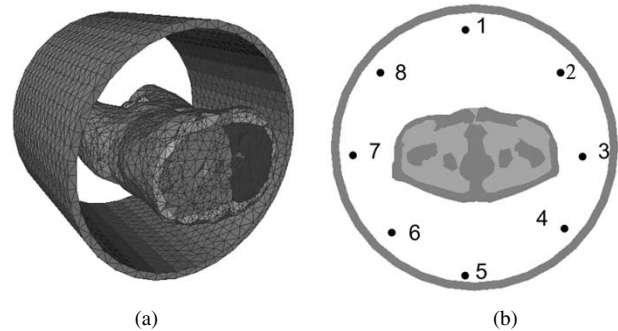
Fig. 2. APA applicator A2: (a) 3-D mesh and (b) location of the sources.
