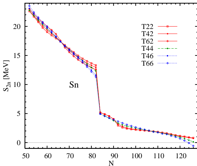
FIG. 30: (Color online) Two-neutron separation energy along the chain of isotopes ( Z = 50 ).
