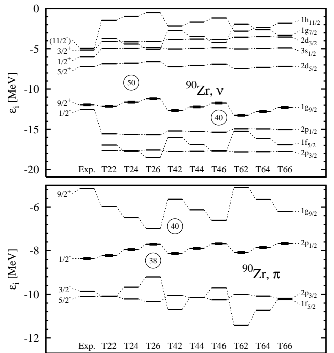
FIG. 23: Same as Fig. 17 for ^{90}\text{Zr} .
