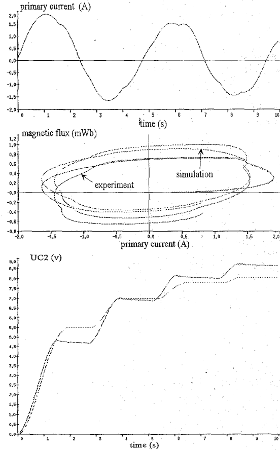
Fig. 8. 200 Hz sine excitation, capacitor voltage and dynamic characteristic for the fault detector circuit of Fig. 7.
