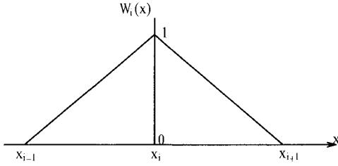
Fig. 4. Distribution function W_i(x) used in the FEM.
