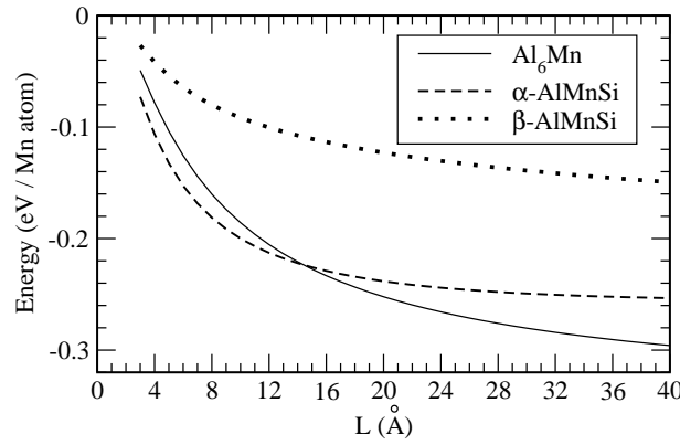
Figure 3: Variation of the band energy due to the effective Mn–Mn interaction in \alpha - \text{Al}_6\text{Mn} , \alpha - \text{AlMnSi} and \beta - \text{Al}_9\text{Mn}_3\text{Si} . [20]
