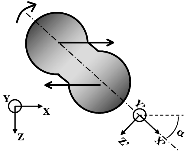
FIG. 7: Description of the two frames used in non central collisions.
