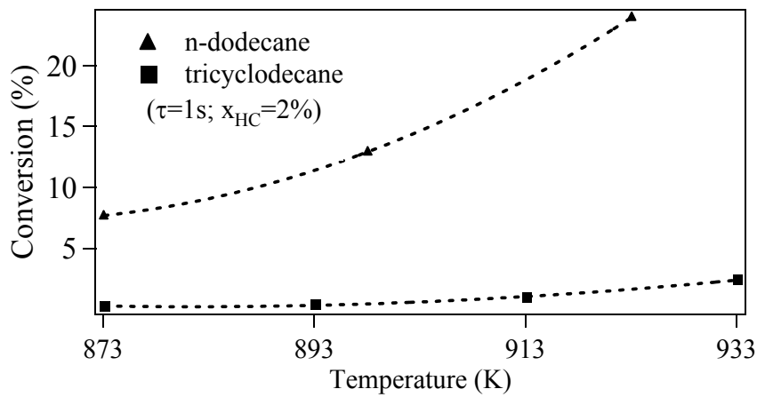
Figure 2: Conversion of tricyclodecane vs. residence time at several temperatures for an initial hydrocarbon mole fraction of 4 % (fig. 2a) and vs. temperature at a residence time of 1s and for several initial hydrocarbon mole fractions (fig. 2b). Comparison with the experimental conversion of n-dodecane (14) vs. temperature at a residence time of 1s and 2 % initial hydrocarbon mole fraction (fig. 2c).
