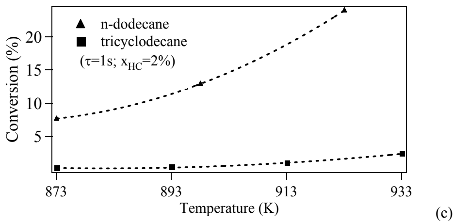
Figure 2: Conversion of tricyclodecane vs. residence time at several temperatures for an initial hydrocarbon mole fraction of 4 % (fig. 2a) and vs. temperature at a residence time of 1s and for several initial hydrocarbon mole fractions (fig. 2b). Comparison with the experimental conversion of n-dodecane (14) vs. temperature at a residence time of 1s and 2 % initial hydrocarbon mole fraction (fig. 2c).
