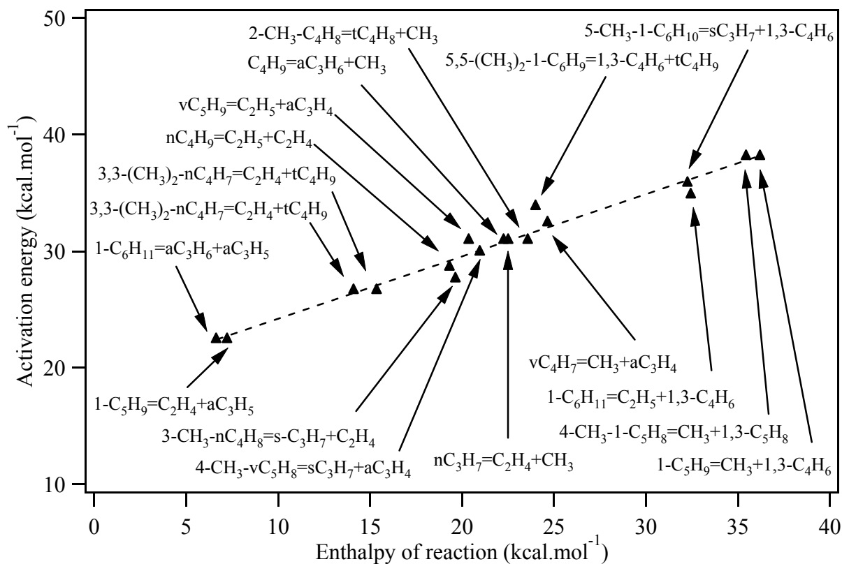
Figure 11: Activation energy of \beta -scission decomposition of acyclic compounds E_{a(\text{acyclic } \beta\text{-scission})} VS.
