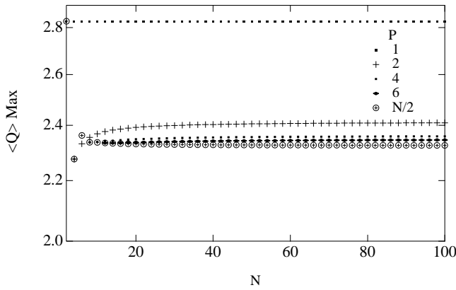
FIG. 1: The maximum of the quantum average \langle Q \rangle for Alice doing P experiments and Bob N - P , as a function of the total number of particles N . The usual Bell situation is obtained for N = 2, P = 1 . Local realist theories predict an upper limit of 2; large violations of this limit are obtained, even with macroscopic systems ( N \rightarrow \infty ). If P = 1 , the violation saturates the Cirel'son limit for any N .
