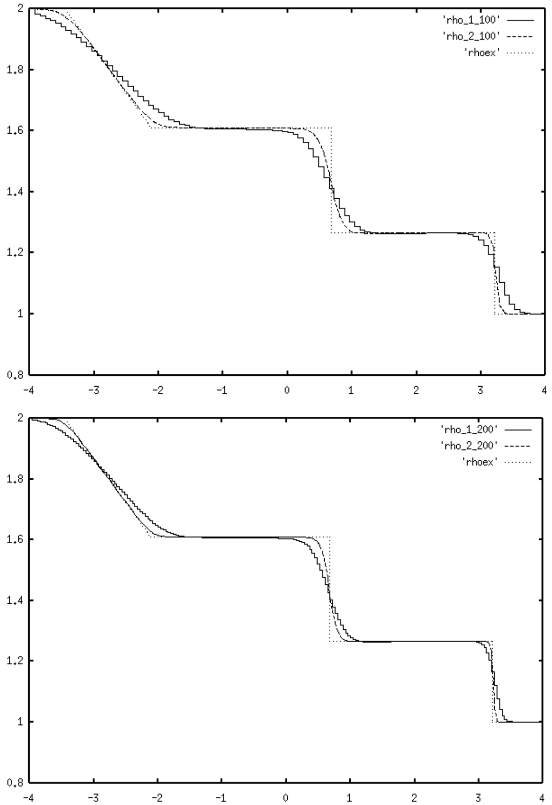
FIGURE 1. Density. First or second order. 100 or 200 cells.
