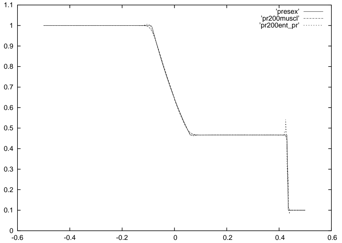
FIGURE 6. Comparison entropic scheme-MUSCL Hancock scheme.
