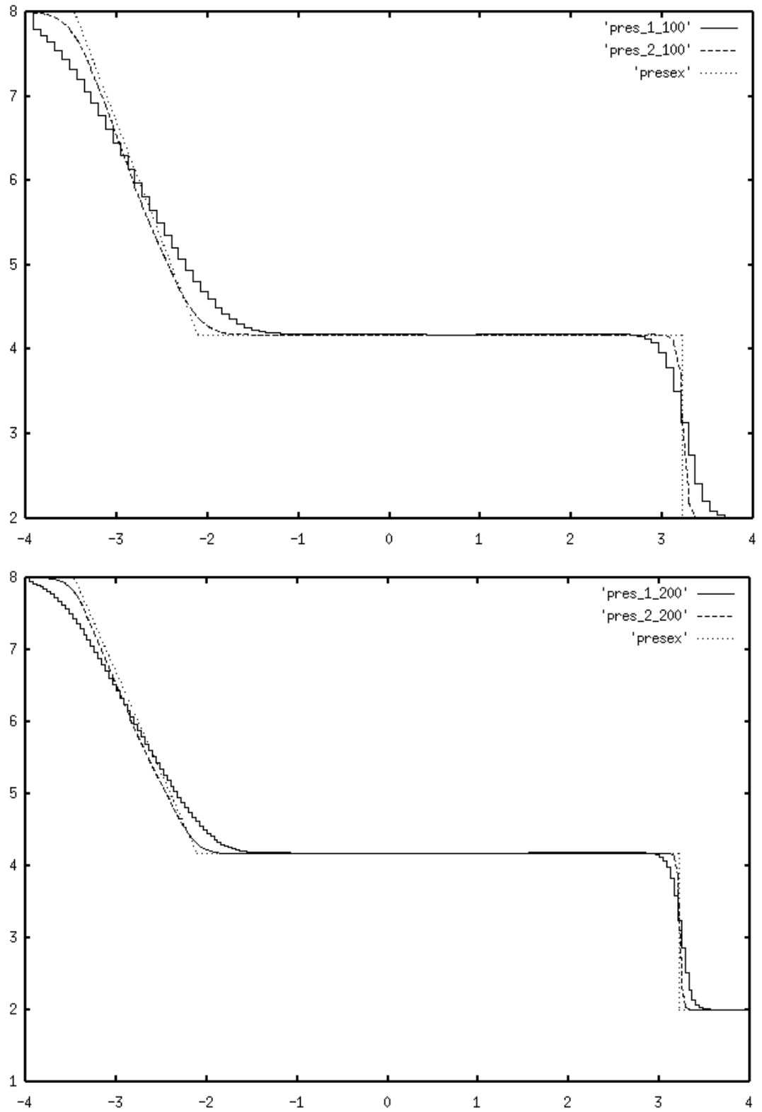
FIGURE 3. Pressure. First or second order. 100 or 200 cells.
