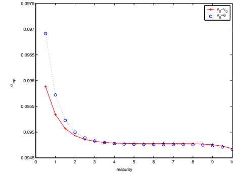
Figure 4: \rho = 0.5 , T \mapsto \sigma_{\text{imp}}(50, T)
