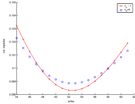
Figure 1: \rho = 0, K \mapsto \sigma_{\text{imp}}(K, 1)
