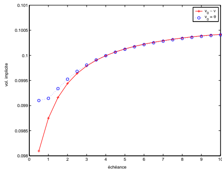
Figure 3: \rho = 0, T \mapsto \sigma_{\text{imp}}(50, T)
