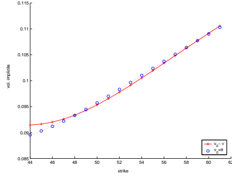
Figure 2: \rho = 0.5, K \mapsto \sigma_{\text{imp}}(K, 1)
