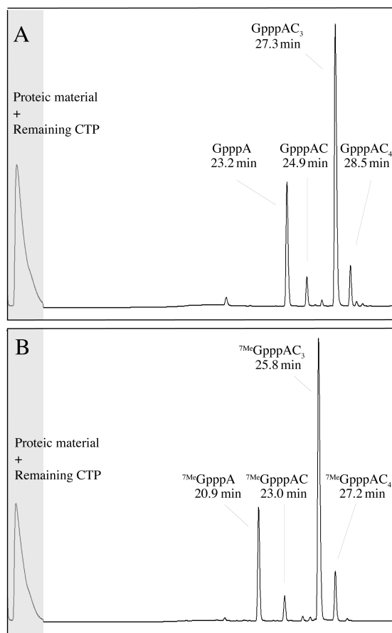
Figure 1. HPLC profiles of T7 DNA primase reaction mixtures using DNA template CCCC GGT TCT 25 . Crude enzymatic mixtures were analyzed directly. Reaction conditions were as follows: T7 DNA primase reaction buffer, DTT and BSA as given in Material and Methods, 5 mM CTP, 1 mM GpppA (A) or 7 MeGpppA (B), 10 μM DNA template CCCC GGT TCT 25 (named dAC3) and 4 μM T7 DNA primase. Reactions were incubated at 37°C for 6 h. The first section (marked in gray) denotes the removal of proteic material and remaining CTP by an on-line cleaning procedure using a pre-column. The produced capped RNAs were then separated on the reverse-phase C18 column. The gradient started after 5 min at 100% eluent A with an increase to 10% eluent B after 25 min, reaching 30% after 35 min and 50% after 40 min.
