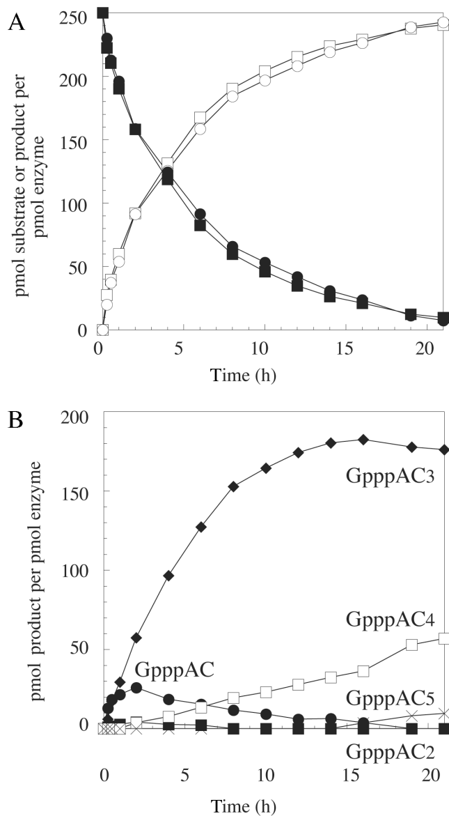
Figure 2. Time course of capped RNA synthesis by T7 DNA primase on DNA template dAC3 (CCCC GGT TCT 25 ). Reaction conditions are given in the legend of Figure 1. Samples were taken at the given time points and analyzed by HPLC. The determination of yields (pmol product per pmol enzyme) is detailed in Material and Methods. (A) global analysis of substrate depletion (■ GpppA, ● 7 MeGpppA) and product generation (□ GpppAC n , ○ 7 MeGpppAC n ) with time, (B) formation of individual products in the GpppA-capped RNA product mixture (● GpppAC, ■ GpppAC 2 , ◆ GpppAC 3 , □ GpppAC 4 , × GpppAC 5 ).
