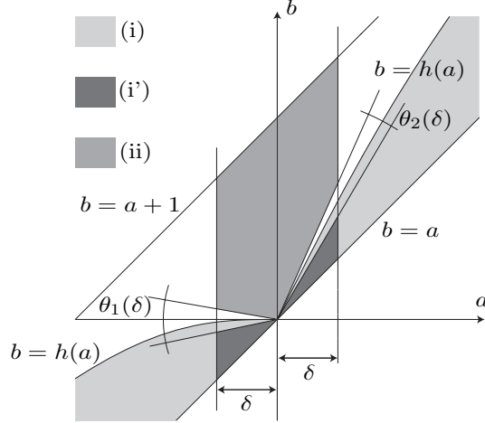
FIGURE 1. Radial symmetry occurs in Region (ii). Optimal functions are not radially symmetric in Region (i), and in particular in Region (i'). The angles \theta_1(\delta) and \theta_2(\delta) are such that \lim_{\delta \rightarrow 0^+} \theta_k(\delta) = 0 for k = 1, 2 .
