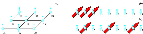
FIG. 2: An array of 3 \times 3 implemented by a linear trap with 9 ions. To generate the interaction in row 1 (insert a) one applies laser light to ions 1, 2, 3 (insert b) while column 2 interaction requires light on ions 2, 5 and 8. (insert c). The advantage of this scheme is that it does not require micro trap fabrication. However, it becomes difficult to implement for large arrays ( N > 3 ) because the distance between the ions in the center of the array gets smaller making their individual addressing difficult.
