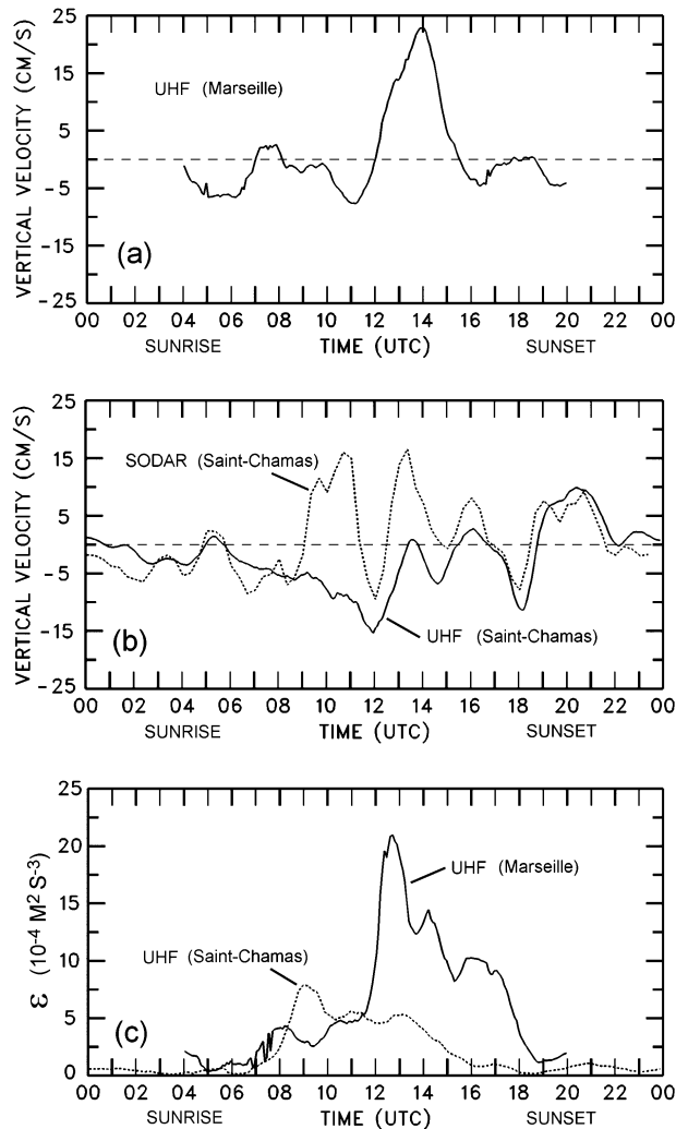
FIG. 4. Mean time series averaged over 7 days of sea-land-breeze circulation and over the height interval 0.3–0.6 km obtained in Jun 2001 during the ESCOMPTE-01 campaign. Vertical velocity time series of (a) the UHF profiler of Marseille and (b) the sodar and UHF profiler of Saint-Chamas. (c) Dissipation rate of turbulent kinetic energy \epsilon deduced from the observations of the two UHF wind profilers. A running average over 3600 s was also applied.
