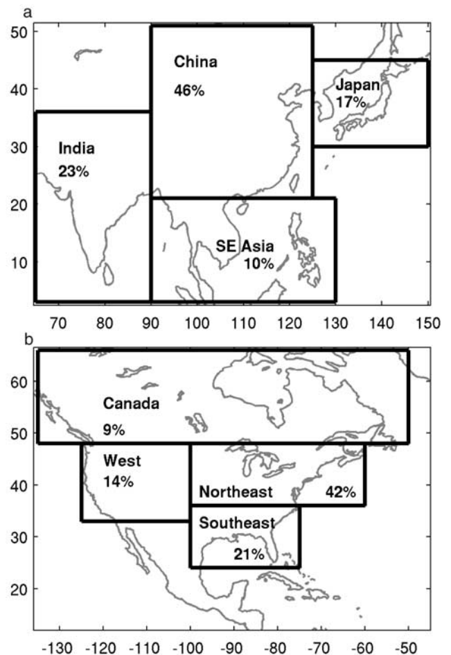
Figure 11. Subregions of (a) Asia and (b) North America. Numbers indicate the percent of Asian or North American NO x emitted within each subregion.
