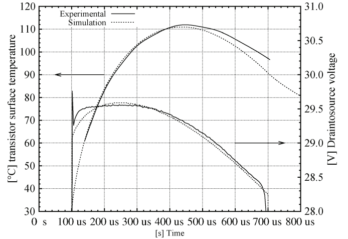
Fig. 13. Comparison between experimental and simulated drain-to-source voltage and transistor temperature during avalanche.
