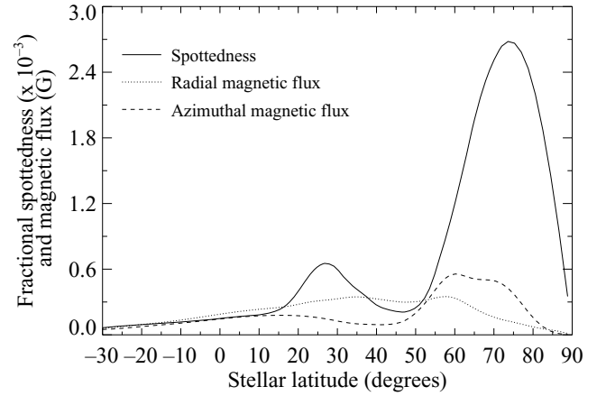
Figure 3. Fractional spottedness and magnetic flux versus stellar latitude for HD 171488. Fractional spottedness/magnetic flux is based on the average spot occupancy/absolute value of the magnetic field at each latitude and is defined by equation (2).
