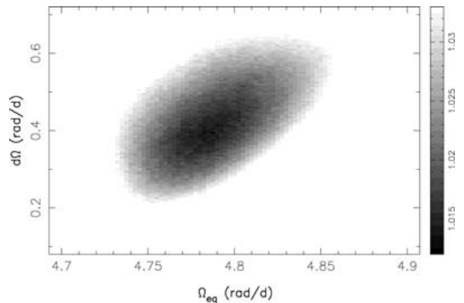
Figure 5. Surface differential rotation \chi^2 minimization for HD171448, 2004 September 24–28. The image shows the reduced- \chi^2 values obtained from the maximum-entropy imaging code for various values of \Omega_{\text{eq}} and d\Omega given a fixed spot coverage of 0.055 and an inclination angle of 60^\circ . Darker regions correspond to lower reduced- \chi^2 values. The grey-scale image projects \pm 5\sigma on to the axes in both \Omega_{\text{eq}} and d\Omega .
