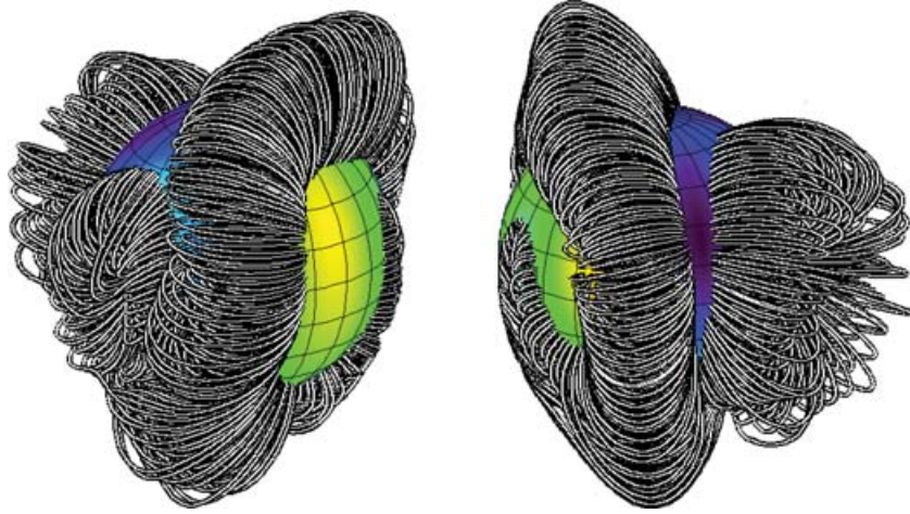
Figure 11. Closed magnetic field lines of the extended magnetic configuration of \tau Sco, extrapolated from the photospheric map of Fig. 8. The star is shown at phases 0.25 (left-hand panel) and 0.83 (right-hand panel). Note the warp of the magnetic equator and the additional networks of closed loops around phase 0.65 (mostly visible on the right-hand side of the right-hand panel).
