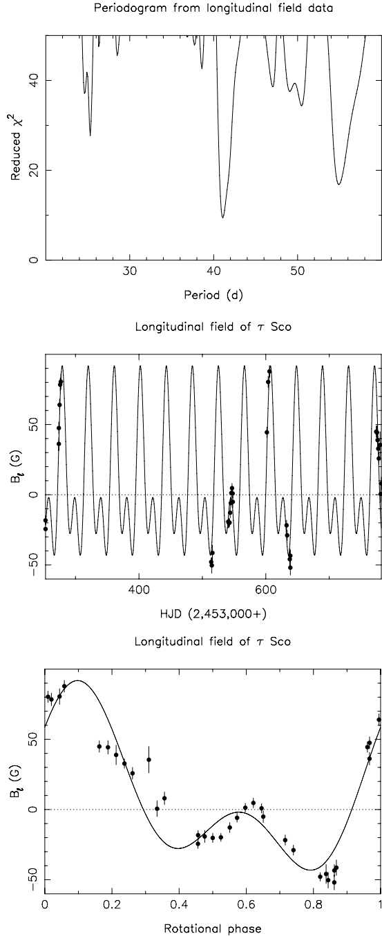
Figure 2. Periodogram resulting from a double sine-wave fit to the longitudinal-field data of \tau Sco. Top panel: \chi^2_r as a function of the period of the main sine wave. A clear minimum is obtained for a period of about 41 d. Middle panel: temporal fluctuations of the longitudinal field of \tau Sco (full dots, with 1\sigma error bars) along with the model fit (full line) for the adopted period of 41.033 d, as a function of heliocentric Julian date (HJD). Bottom panel: as for the middle panel, but as a function of rotation phase, computed using the ephemeris of equation (1).
