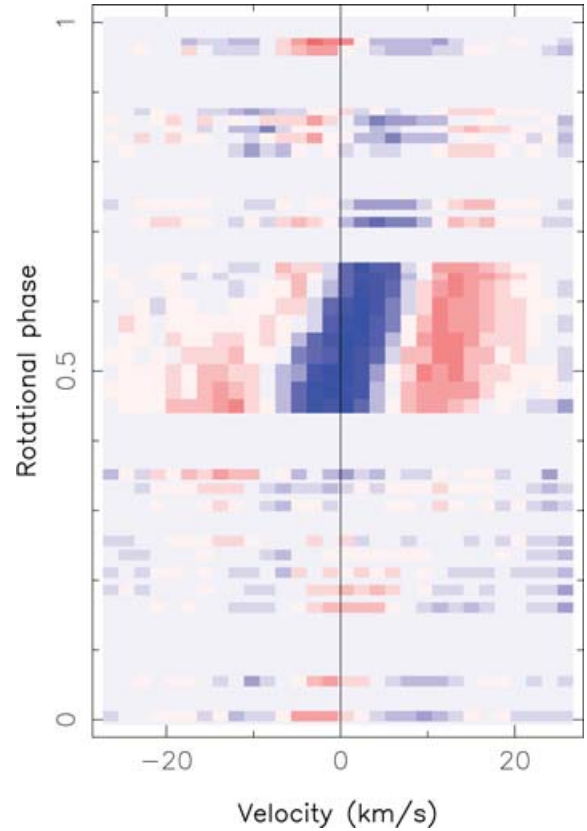
Figure 6. Dynamic LSD Stokes I spectrum of \tau Sco, demonstrating that the average unpolarized line is also modulated with the detected rotation period of 41 d (see Section 3). A simple synthetic profile (featuring Gaussian turbulence broadening with an FWHM of 13.5 \text{ km s}^{-1} and v_e \sin(i) = 6 \text{ km s}^{-1} , see the text) was removed from all profiles to emphasize variability. A clear signal, centred at phase 0.5, crosses the line profile and indicates that the average photospheric line of \tau Sco gets slightly narrower (by about 10 per cent) around phase 0.5. Blue and red, respectively, correspond to line-absorption/emission features with an amplitude of \pm 0.4 per cent of the continuum intensity (i.e. \pm 3 per cent of the central line depth).
