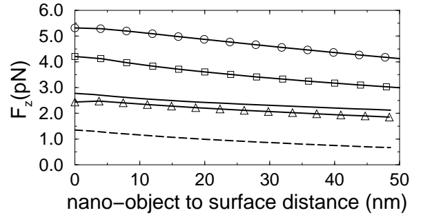
FIG. 5. z component of the force experienced by a particle as a function of the distance between the particle and the substrate under TM illumination. The particle is placed at the apex of the probe. Solid line : sphere ( \epsilon = 2.25 , radius: 10 nm, \theta = 43^\circ ). Dashed line: sphere ( \epsilon = 2.25 , radius: 10 nm, \theta = 50^\circ ). Circles : sphere ( \epsilon = 2.25 , radius: 30 nm, \theta = 50^\circ ). Triangles (force \times 0.1 ): sphere of gold ( \epsilon = -2.81 + 3.18i , radius: 10 nm, \theta = 50^\circ ). Squares : cube ( \epsilon = 2.25 , size: 20 nm, \theta = 50^\circ ).
