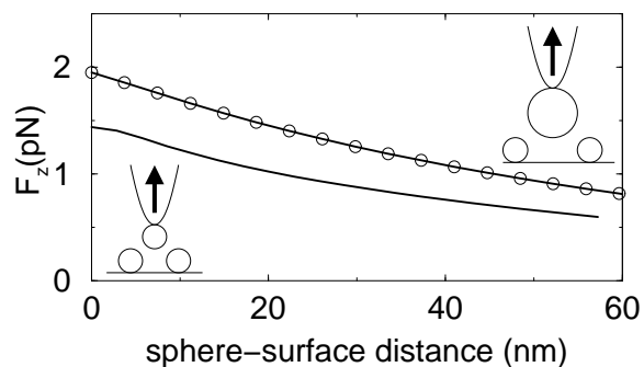
FIG. 7. Force along z as experienced by the middle sphere (solid line) versus vertical position of the middle sphere trapped at the apex probe ( \theta = 50^\circ ). Solid line : sphere with a 10 nm radius. Circles : sphere with a 20 nm radius.
