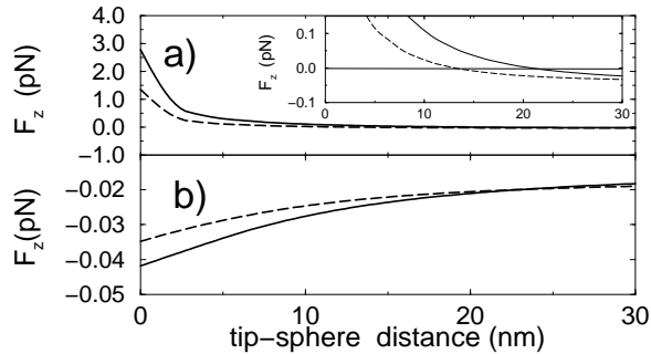
FIG. 2. z component of the force experienced by the sphere versus the distance between the tip and the sphere. Solid line : \theta = 43^\circ . Dashed line : \theta = 50^\circ . a) TM polarization. b) TE polarization.
