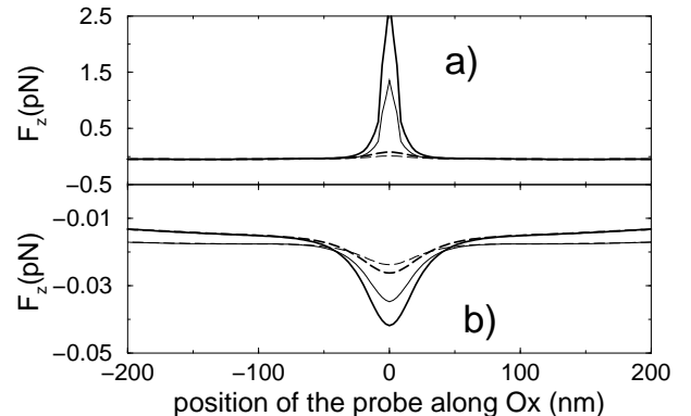
FIG. 3. Force along z experienced by the sphere as a function of the lateral position of the probe. The sphere is at the origin. a) TM polarization, b) TE polarization. Thick lines : \theta = 43^\circ . Thin lines : \theta = 50^\circ . The tip is either 20 nm (solid lines) or 31 nm (dashed lines) above the substrate.
