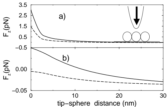
FIG. 6. Force along z versus vertical position of the probe for three spheres aligned along x . The probe is centered over the middle sphere. Solid line \theta = 43^\circ . Dashed line \theta = 50^\circ . a) Force on the middle sphere. b) Force experienced by the spheres on the sides.
