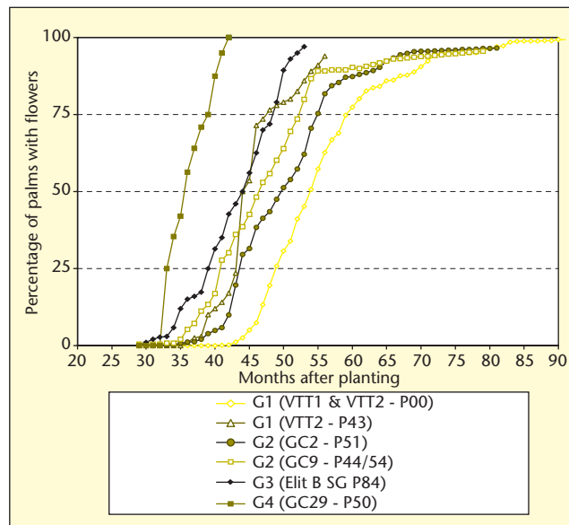
Figure 5. Vanuatu Tall flowering for different generations.
