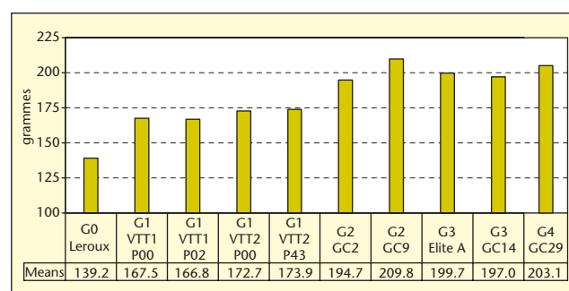
Figure 8. Copra content of the nuts (C/N) for different Vanuatu Tall generations.
