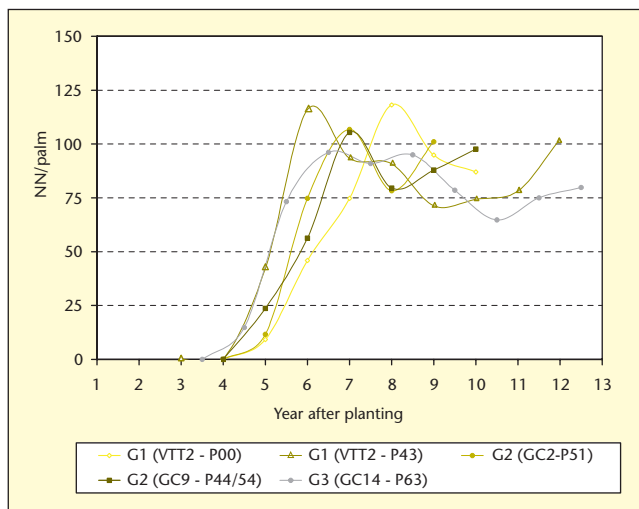
Figure 9. Nut yields per palm for the different VTT generations over time.
