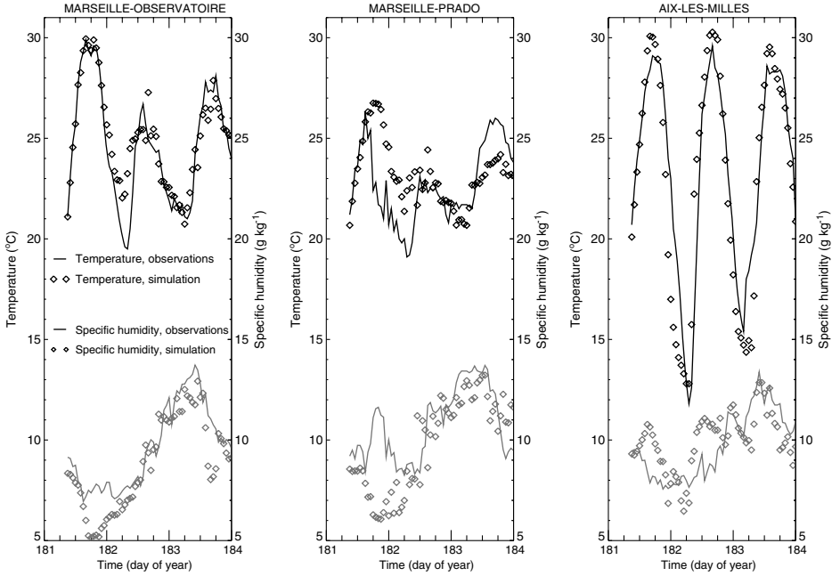
Figure 8. Comparison between observations and simulation of temperature (black) and specific humidity (grey) at 2 m for three locations: Marseille-Observatoire (left), Marseille-Prado (middle) and Aix-les-Milles (right).
