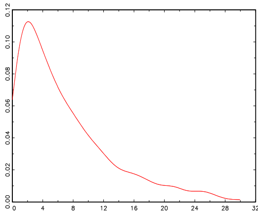
Figure 4: Monte-Carlo distribution for the time to run over \mathbf{u} for the Adult female (15-45) subpopulation ( \mathbf{u} = X_{\text{ref},0.7} = 6.42 \mu\text{g}/\text{kgbw} , with x_0 = 2.92 ).
