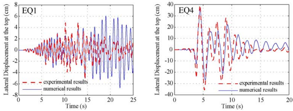
Figure 2.8. Lateral displacements at the top versus time for EQ1 and EQ4. Experimental (dashed lines) and numerical results (continuous lines).
