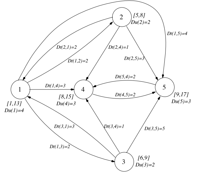
Figure 4: Graph representing five candidate images
