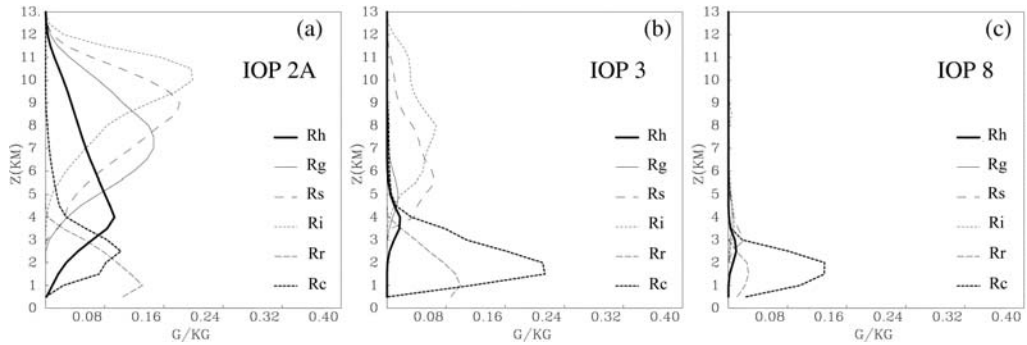
Figure 12. Mean vertical structure of the hydrometeors computed in the budget box shown in Fig. 1(b) for (a) IOP 2A, averaged between 2000 and 2015 UTC on 17 September 1999, (b) IOP 3, averaged between 1830 and 1845 UTC on 25 September 1999, and (c) IOP 8, averaged between 1700 and 1715 UTC on 20 October 1999. R_h , R_g , R_s , R_i , R_r , and R_c denote the mixing ratios of hail, graupel, snow/agggregates, pristine ice, rain water, and cloud water respectively.
