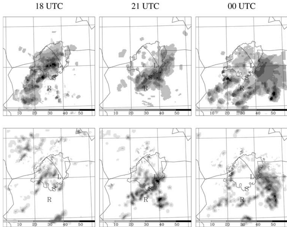
Figure 6. Time evolution of the radar reflectivity (dBZ) at 2000 m for IOP 2A from 18 UTC on 17 September to 00 UTC on 18 September. The upper row shows observed fields from the radar composite, and the lower row the results from the simulation. The closed contour indicates the limits of the Toce-Ticino watershed. The other lines approximately represent the borders between France, Italy and Switzerland. The locations of the Monte Lema, S-Pol and Ronsard radars are indicated by the letters L, S, and R respectively.
