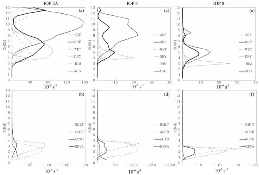
Figure 13. Mean vertical structure of the main microphysical processes involved in IOP 2A; normalized sources acting on (a) the solid precipitation ( R_s + R_g + R_h , see text) with groupings DRY^a , RIM^b , AUG^c , DEP^d and ACC^e , and on (b) the liquid precipitation ( R_r ) with ACCR^f , AUTO^g , REVA^h , RMLT^i . Groupings are formed from processes marked by corresponding superscripts in Table 2. The averaging periods are the same as in Fig. 12. (c, d) and (e, f) are as (a, b), but for IOPs 3 and 8, respectively.
