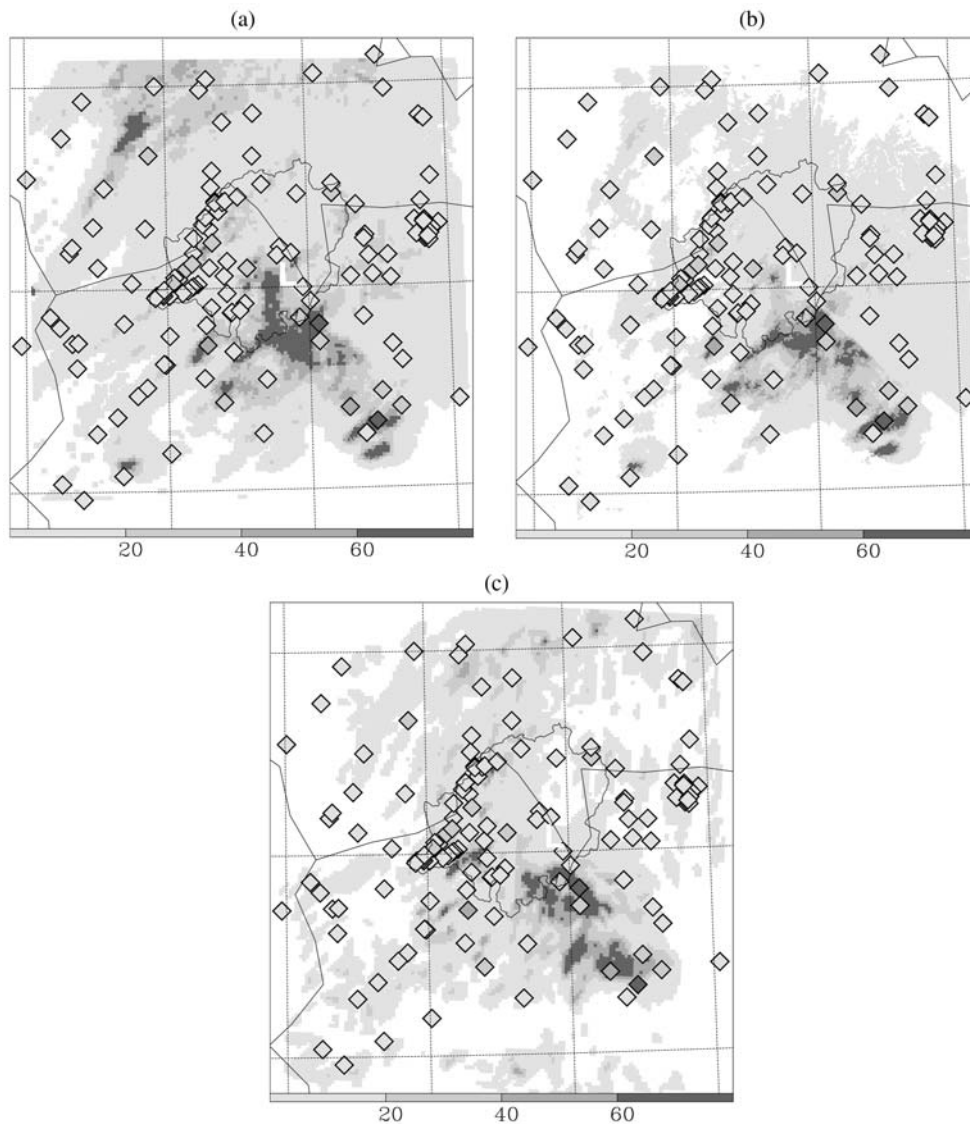
Figure 8. 12-hour accumulated precipitation (shading, mm) from 12 UTC on 17 September 1999 (a) deduced from the Alpine radar composite, (b) deduced from the RAIN data product, and (c) computed in the 2 km grid-mesh domain. The corresponding raingauge measurements (diamonds) are superimposed on each plot.
