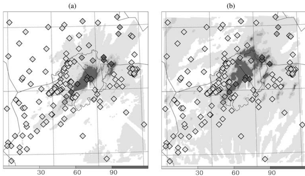
Figure 10. 24-hour accumulated precipitation (shading, mm) from 12 UTC on 25 September (a) deduced from the RAIN data product and (b) computed in the 2 km grid-mesh domain. L indicates the location of the Monte Lema radar.
