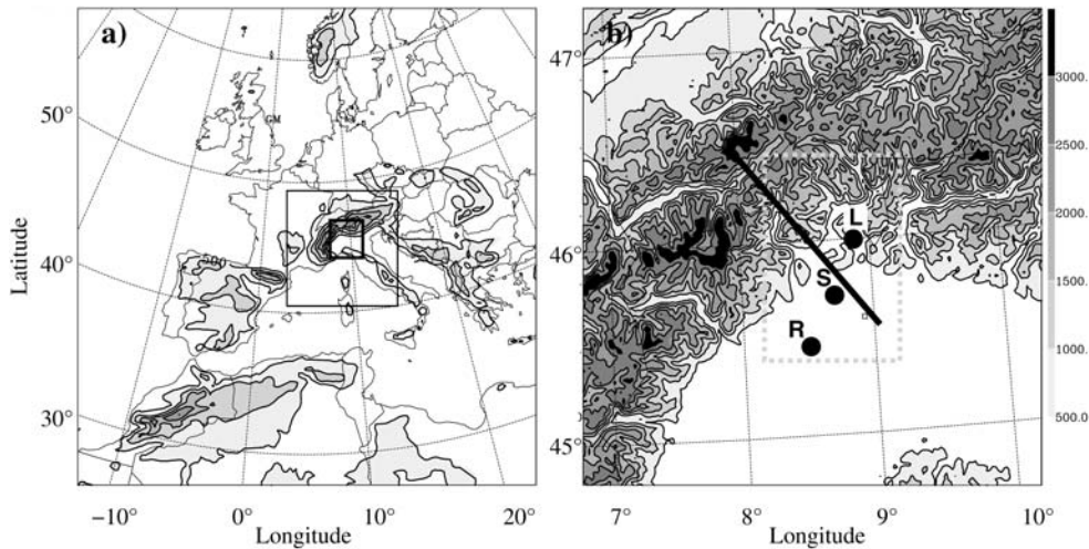
Figure 1. (a) Geographical domains used for the nested simulation. The outer frame shows the 32 km grid-mesh domain and its topography; the location of the 8 km (2 km) grid-mesh domain is indicated by the thin (bold) square. (b) Topography (m) of the 2 km grid-mesh domain, and locations of the three radars (R, S, and L for Ronsard, S-Pol, and Monte Lema respectively). The dashed square denotes the subdomain used for the microphysical budget computation and the bold solid line indicates the location of the vertical cross-section shown in Fig. 7.
