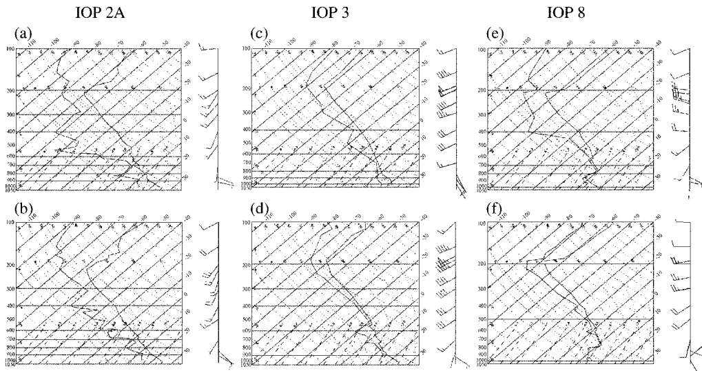
Figure 4. Milano radiosoundings for IOP 2A (17 September 1999) at (a) 12 UTC and (b) 18 UTC. (c, d) and (e, f) are as (a, b), but for IOP 3 (25 September 1999) and IOP 8 (20 October 1999), respectively.
