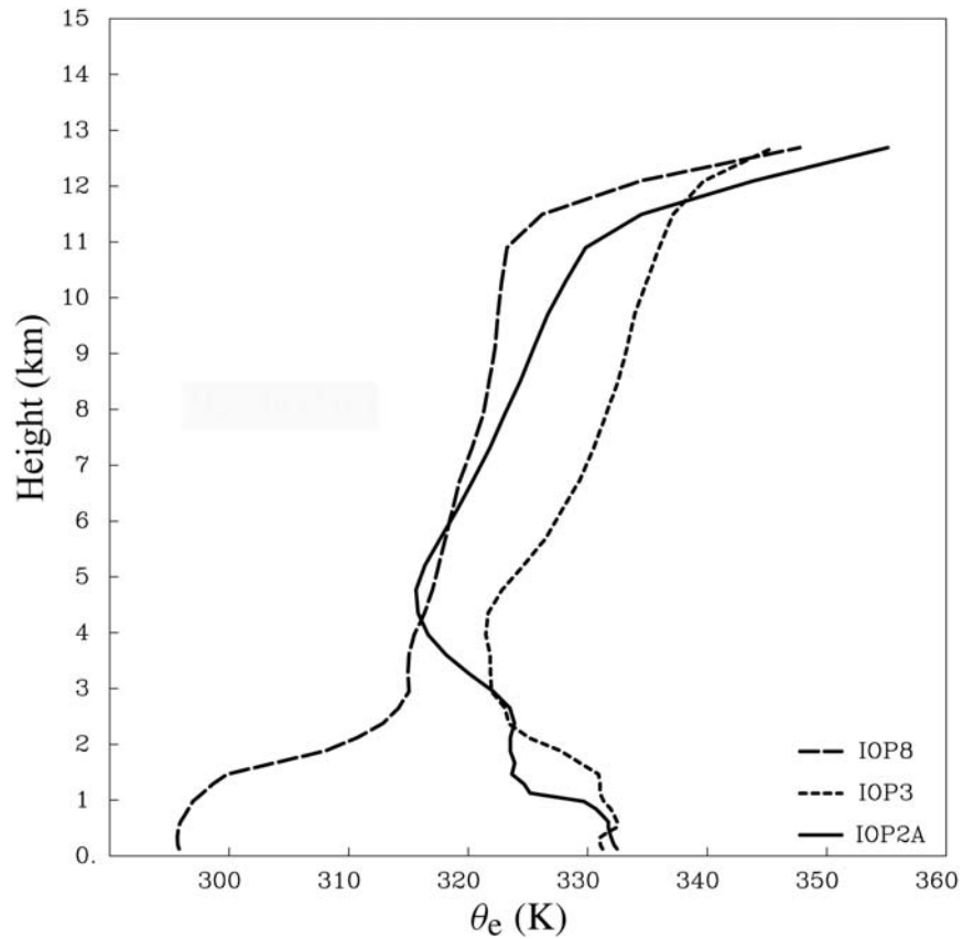
Figure 5. Mean vertical profile of the equivalent potential temperature for IOP 2A, IOP 3, and IOP 8 at Milano-Linate computed in the model and averaged over the first ten hours of each simulation.
