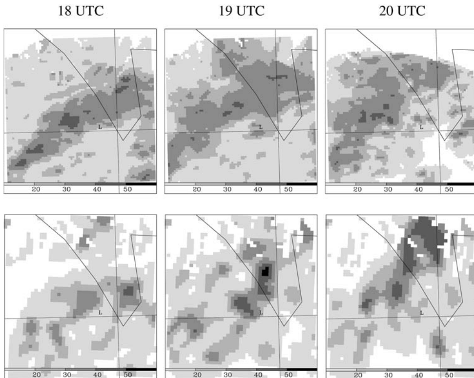
Figure 9. As Fig. 6, but over a smaller domain centred above the Lago Maggiore area and for IOP 3 (18 to 20 UTC on 25 September).
