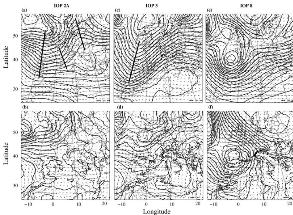
Figure 3. Synoptic situation at 12 UTC on 17 September 1999 (IOP 2A): (a) 500 hPa geopotential height (contour interval 30 m) with wind vectors, and (b) mean-sea-level pressure (contour interval 3 hPa) with surface wind vectors. (c, d) and (e, f) are as (a, b), but for 12 UTC on 25 September 1999 (IOP 3) and on 20 October 1999 (IOP 8), respectively. The bold lines in (a) and (c) indicate the locations of the troughs or ridges mentioned in the text.
