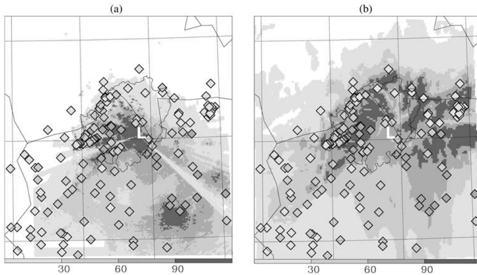
Figure 11. As Fig. 10, but for 00 UTC on 21 October to 00 UTC on 22 October.
