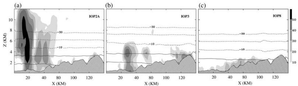
Figure 7. Vertical cross-section of the simulated radar reflectivity (shading, dBZ) and temperature (contours, °C) along the line shown in Fig. 1(b) for (a) IOP 2A (2000 UTC on 17 September 1999), (b) IOP 3 (1830 UTC on 25 September 1999), and (c) IOP 8 (1700 UTC on 21 October 1999).
