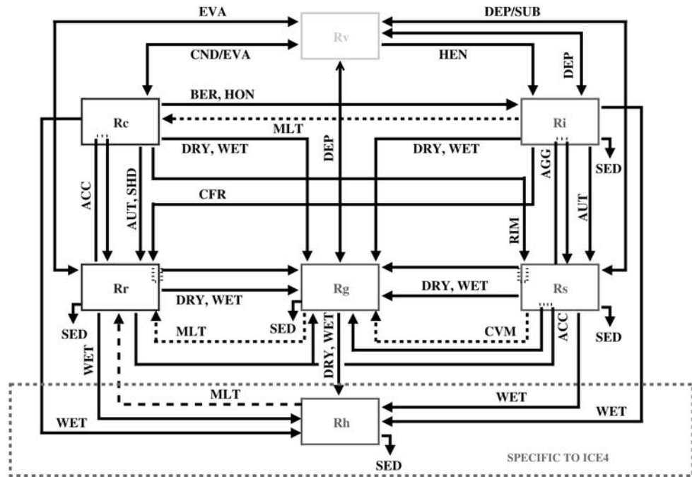
Figure 2. Sketch of the ICE3 and ICE4 microphysical schemes. R_v , R_c , R_r , R_i , R_s , R_g , and R_h refer to the mixing ratios of water vapour, cloud droplets, raindrops, pristine ice, snow/aggregates, graupel, and hail respectively. The different microphysical processes are designated by a group of three letters (EVA, DEP, etc.; see Table 2 for the complete list).
