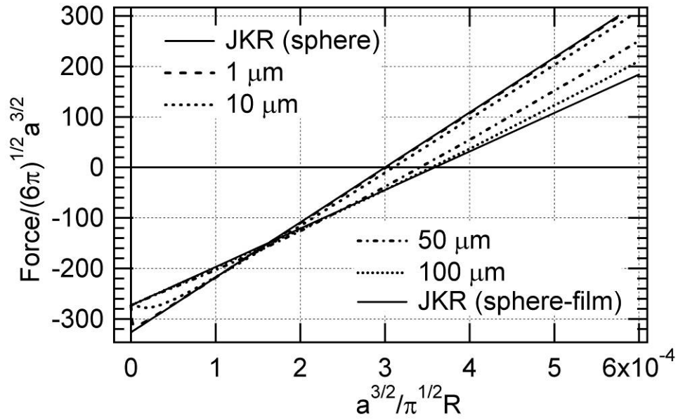
Fig. 4: Reduced JKR plots for various film thicknesses, with the parameters of Tables 1 and 2. Also shown are the JKR asymptotes for a rigid substrate without coating (sphere) and an infinitely thick coating (sphere-film). The JKR (sphere) curve is nearly always coincident to the 1 \mu\text{m} thick film curve, except at very small contact radii. The JKR (sphere-film) curve is coincident to the 100 \mu\text{m} thick film curve except at larger contact radii.
