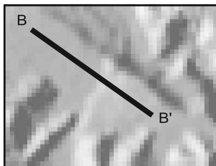
Figure 6. Chushiang fault scarp. This fault disrupts the fill deposit (Figure 5). (left) Shaded DEM clearly revealing the fault scarp in the morphology. (right) Topographic profile across the fault scarp (section B–B').
