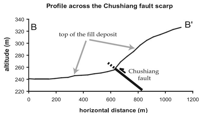
Figure 6. Chushiang fault scarp. This fault disrupts the fill deposit (Figure 5). (left) Shaded DEM clearly revealing the fault scarp in the morphology. (right) Topographic profile across the fault scarp (section B–B').
