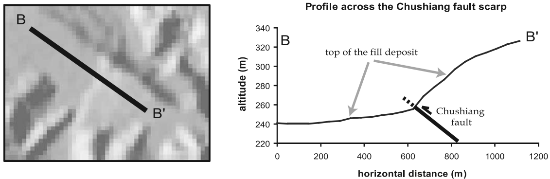
Figure 6. Chushiang fault scarp. This fault disrupts the fill deposit (Figure 5). (left) Shaded DEM clearly revealing the fault scarp in the morphology. (right) Topographic profile across the fault scarp (section B–B').
