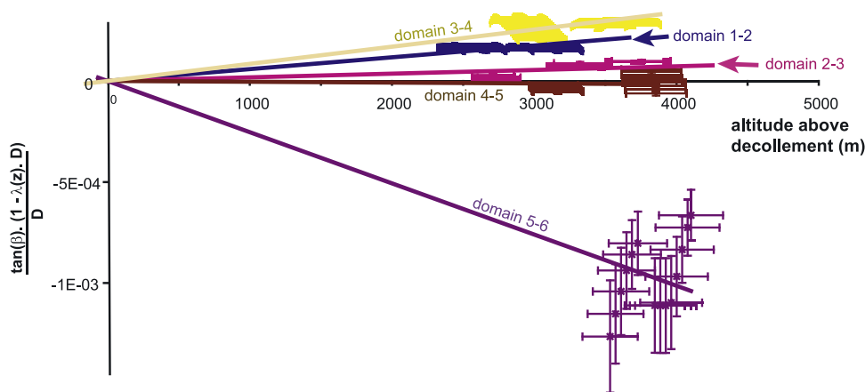
Figure 20. Plot of [\tan(\beta)(1 - \lambda(z)D)]/D as a function of altitude z above the decollement for southern Pakuashan. See Figure 17 caption for further details.
