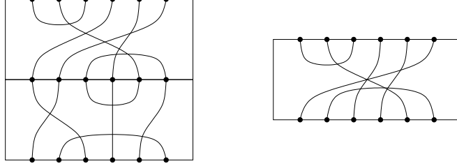
FIGURE 1. Multiplication of two diagrams in the Brauer monoid.
