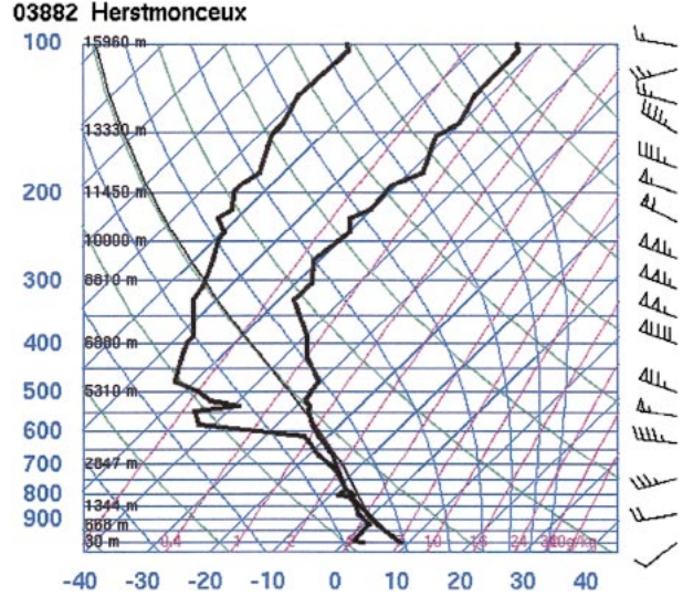
FIG. 5. Radio sounding of Herstmonceux ( 50.90^\circ\text{N} , 0.31^\circ\text{W} ) on 13 Apr 1999 at 1200 UTC. Abscissa is temperature in ^\circ\text{C} , ordinate is pressure in hPa. The wind, on the right part, is given in kt with values of 5, 10, 50 for half barb, full barb, and triangle, respectively.
