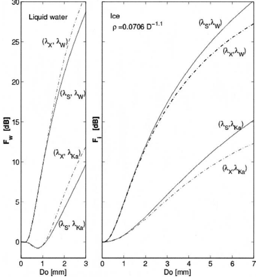
FIG. 1. Variation of the non-Rayleigh scattering term F_{\lambda_i, \lambda_s}(D_0) for water and for ice, written F_w and F_i , respectively, as a function of the mean volume diameter D_0 . Here \lambda_s , \lambda_x , \lambda_{Ka} , \lambda_w are wavelengths for S, X, Ka, and W bands, respectively; \rho is the density in \text{g cm}^{-3} , with D in mm.
